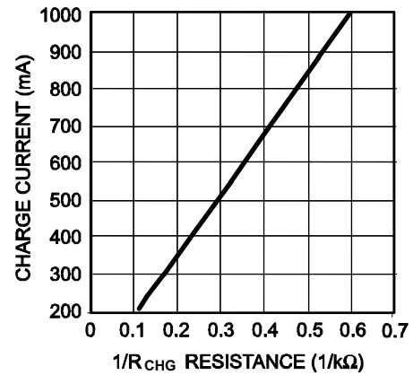
Figure 4—Charge Current vs 1/R_{CHG} Resistance
