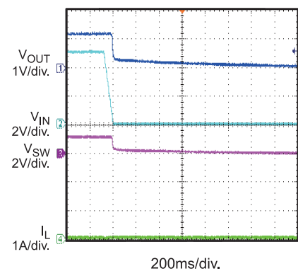
VIN Shutdown without Load
