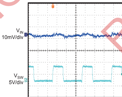
Input Ripple Voltage
