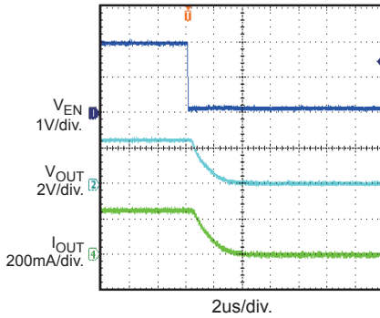
EN Shut Down with Resistive Load I_{OUT}=250mA
