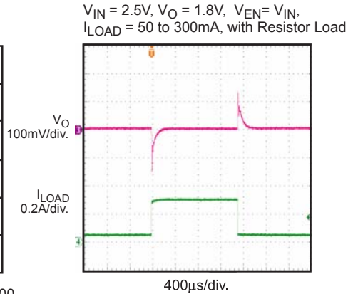
Load Transient
