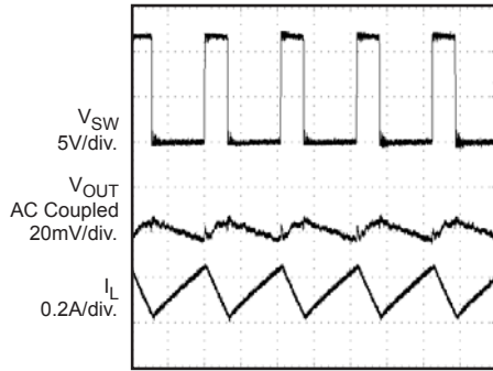
Steady State Operation Backlight Mode
