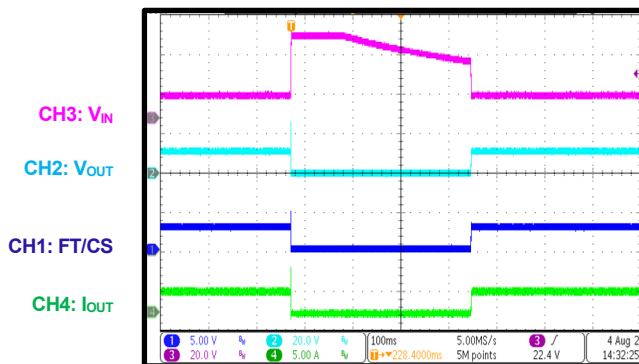
Load Dump
