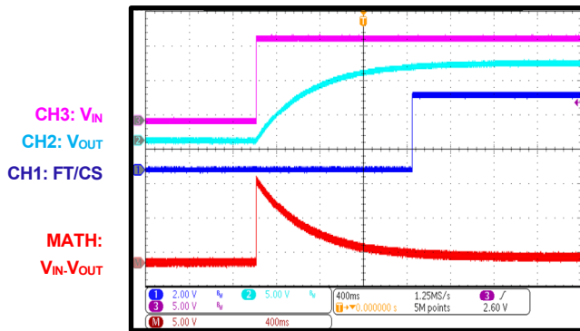
Open-Load Detection
