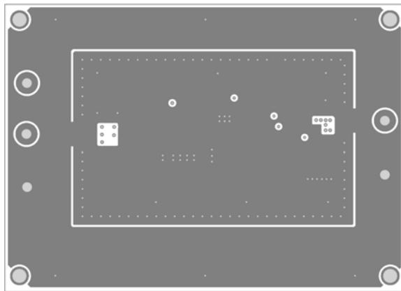
Figure 3—Inner1 Layer
