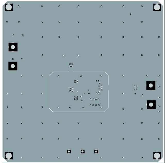
Figure 3: Inner1 Layer
