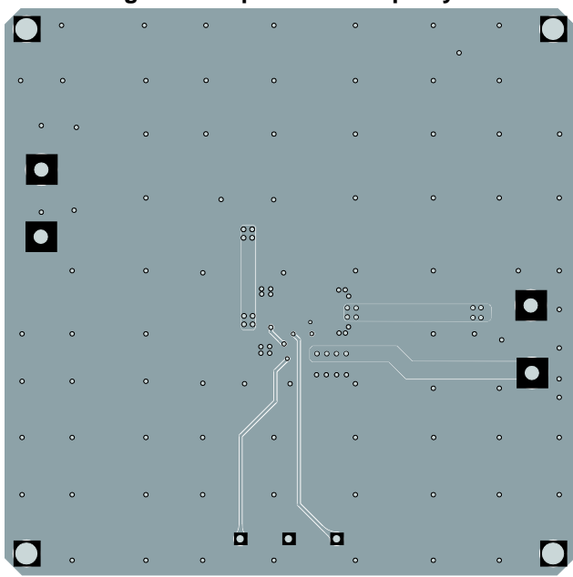
Figure 4: Inner2 Layer
