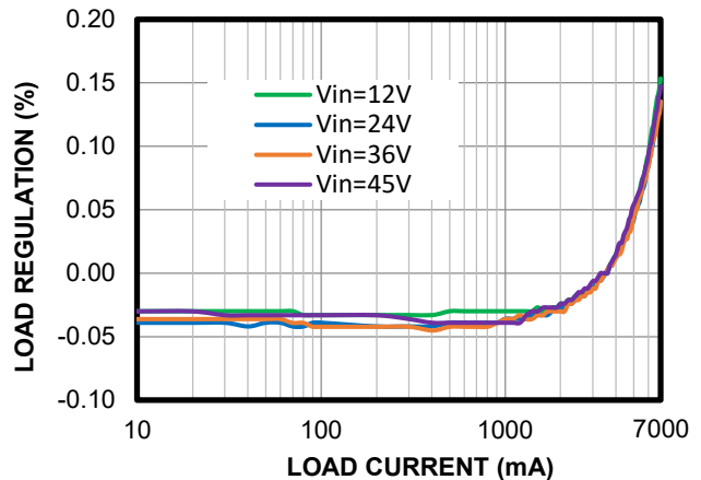
Load Regulation FCCM, V_{OUT} = 3.3V
