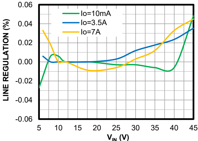
Line Regulation AAM mode, V_{OUT} = 3.3V
