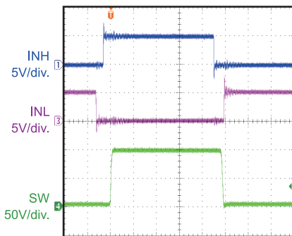
Input Signals and SW Node
