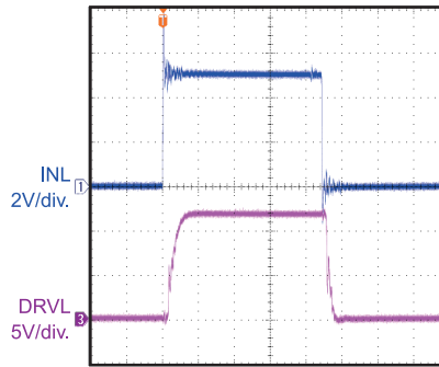
INL to DRVL Delay with MOSFET
