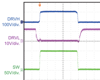
Gate Signals and SW Node
