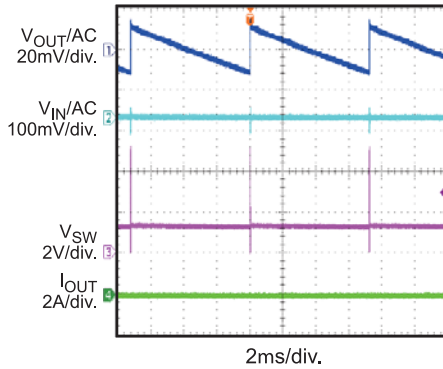
Input and Output Ripple I_{OUT}=0A
