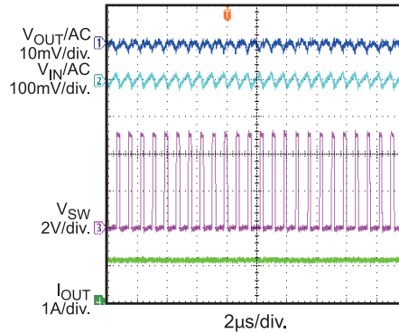
Input and Output Ripple I_{OUT}=1A
