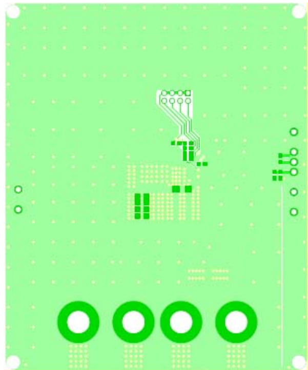
Figure 4: Bottom Layer
