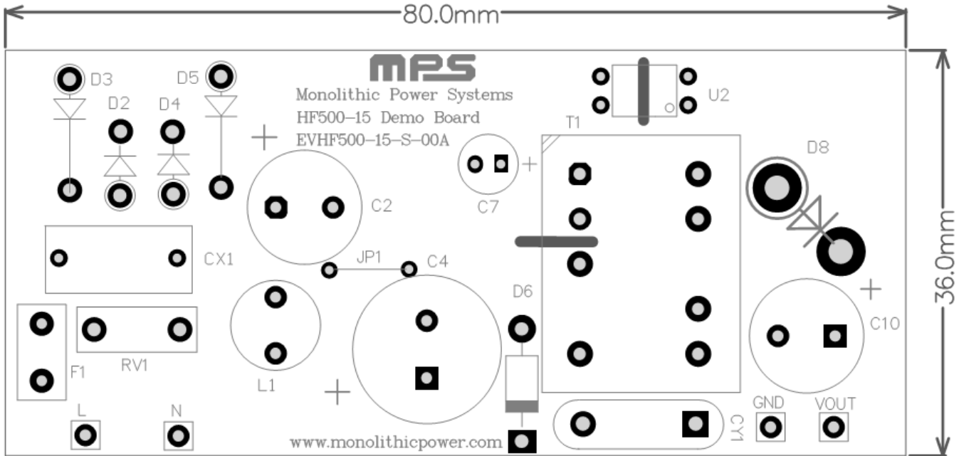
Figure 2: Top Layer
