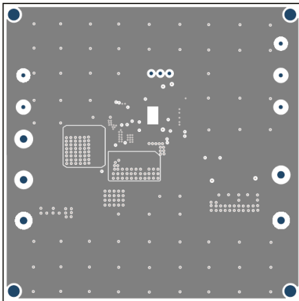
Figure 3—Middle Layer 1
