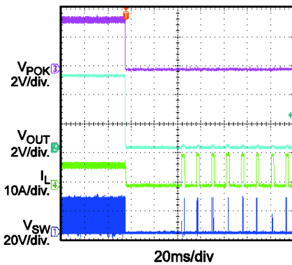
SCP Entry I_{OUT} = 7A to short circuit
