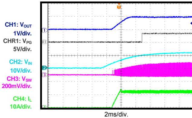
Start-Up through Input Voltage I_{OUT}=12A
