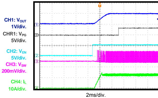
Start-Up through EN I_{OUT}=12A
