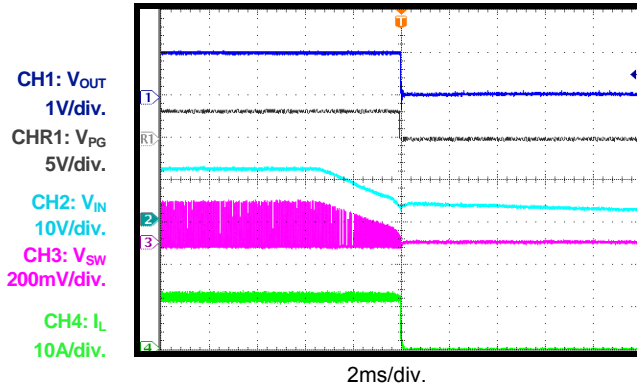
Shutdown through Input Voltage I_{OUT}=12A
