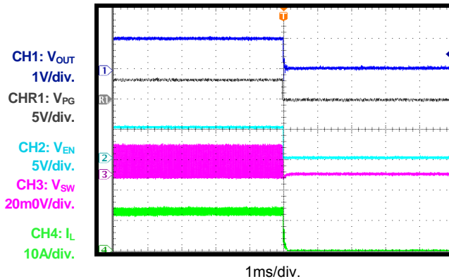
Shutdown through EN I_{OUT}=12A
