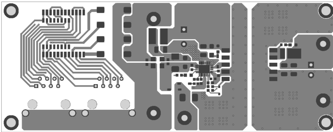
Figure 2: Top Layer
