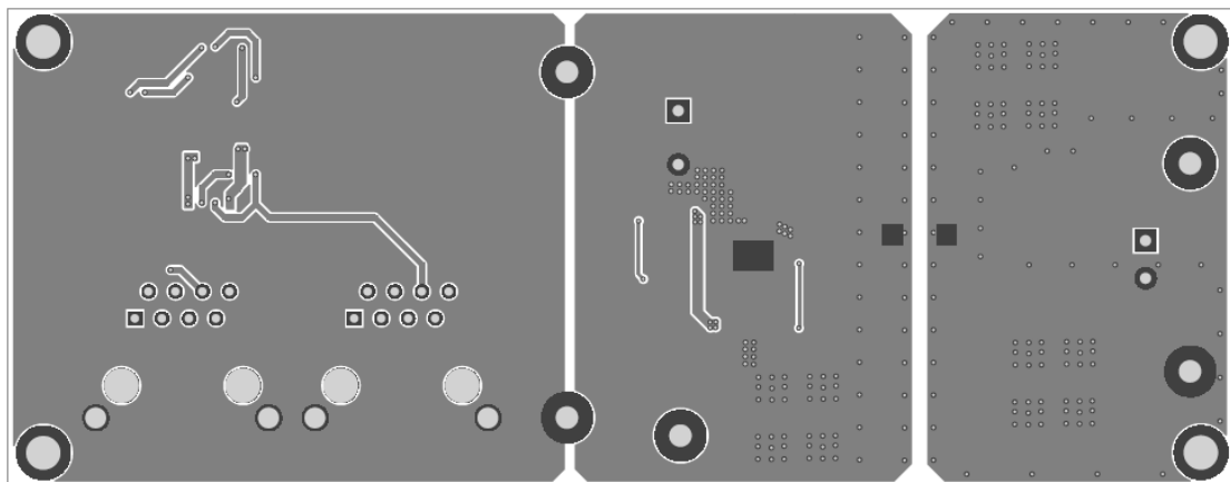
Figure 3: Bottom Layer
