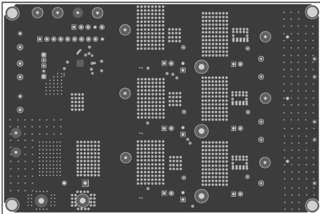
Figure 3: Inner 1 Layer
