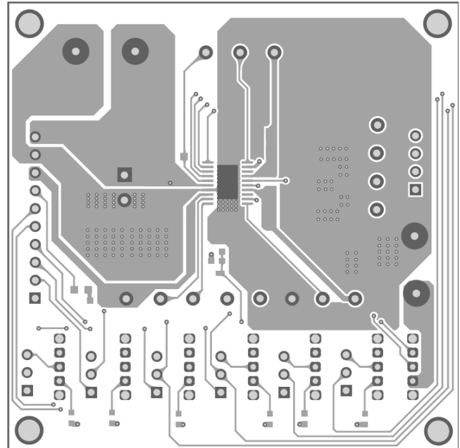
Figure 3: Top Layer
