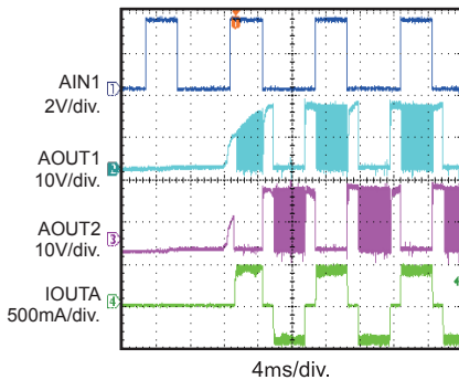
Power Ramp Up-Half Step V_{IN}=15\text{V}
