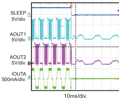
Sleep Entry-Half Step V_{IN}=9\text{V}
