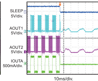
Sleep Entry-Full Step V_{IN}=9\text{V}
