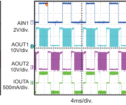
Steady State-Half Step V_{IN}=15\text{V}
