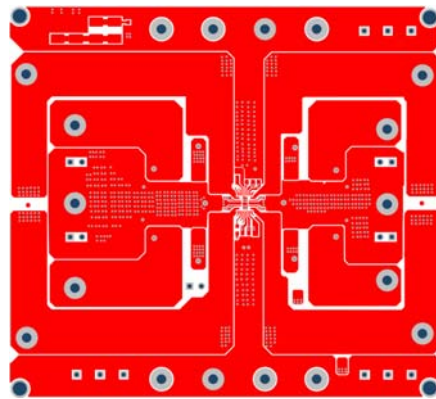
Figure 2: Top Layer
