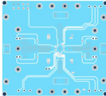
Figure 4: Middle Layer 2
