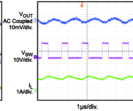
Output Voltage Ripple I_{OUT} = 1A
