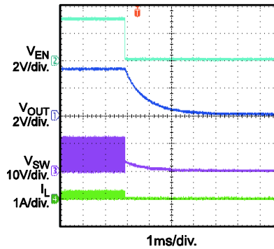
Start Down I_{OUT} = 0.1A
