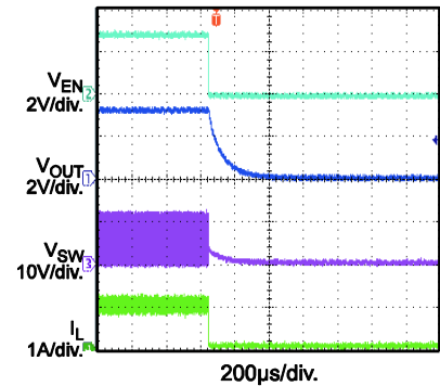
Start Down I_{OUT} = 1A
