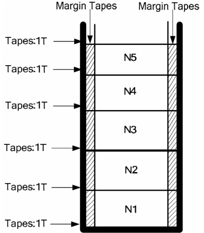
Winding Diagram
