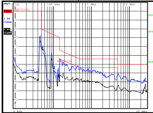
Conduct EMI-L Line V_{IN}=120Vac , 7 LED Output
