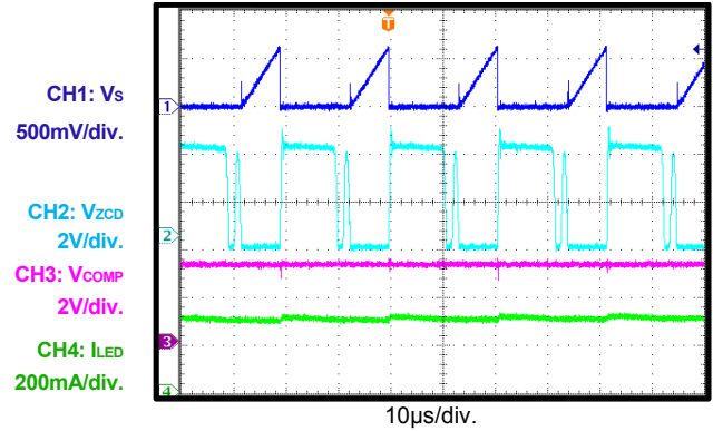
Steady State V_{IN}=120Vac , 7 LED Output
