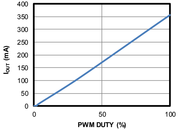
1kHz PWM Dimming Curve V_{IN}=120Vac , 7 LED Output
