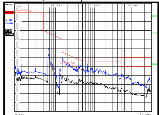
Conduct EMI-N Line V_{IN}=120Vac , 7 LED Output
