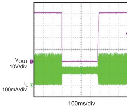
Short Circuit Protection Entry & Recovery
