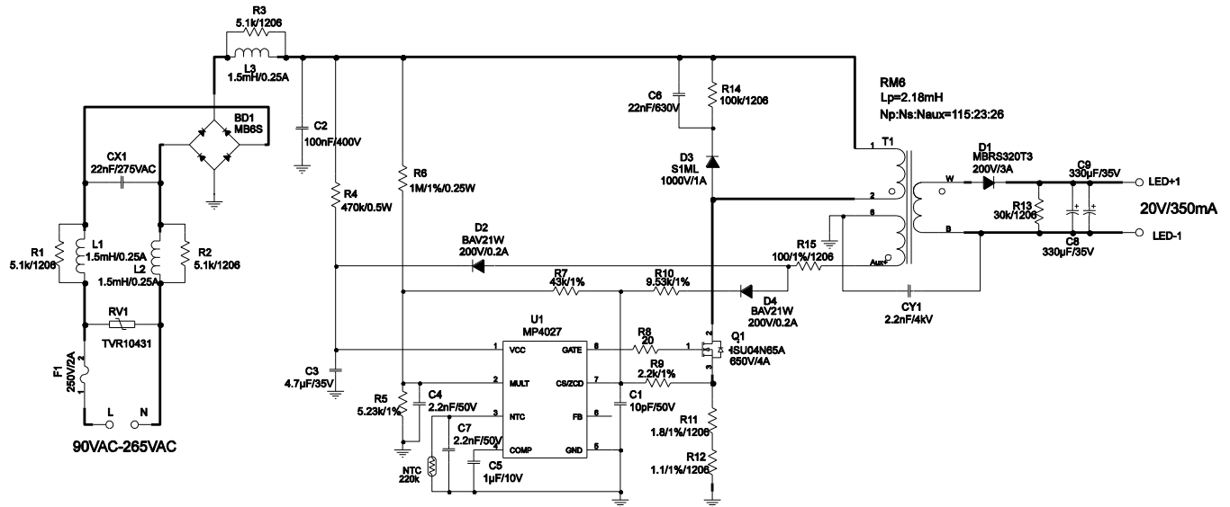
Figure 1 - Schematic
