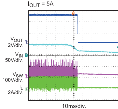
V_{IN} Shutdown
