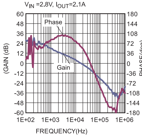
Bode Plot
