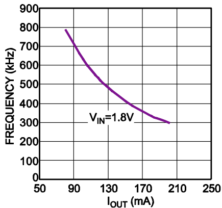
SW Frequency vs. Load Current
