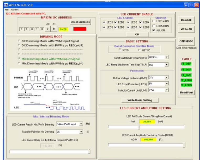
Picture 4—MP3376 GUI Interface
