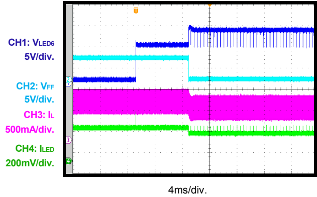
LED Short Protection Short one string when working
