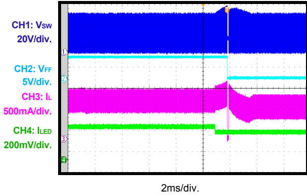
Open LED Protection Open one string when working
