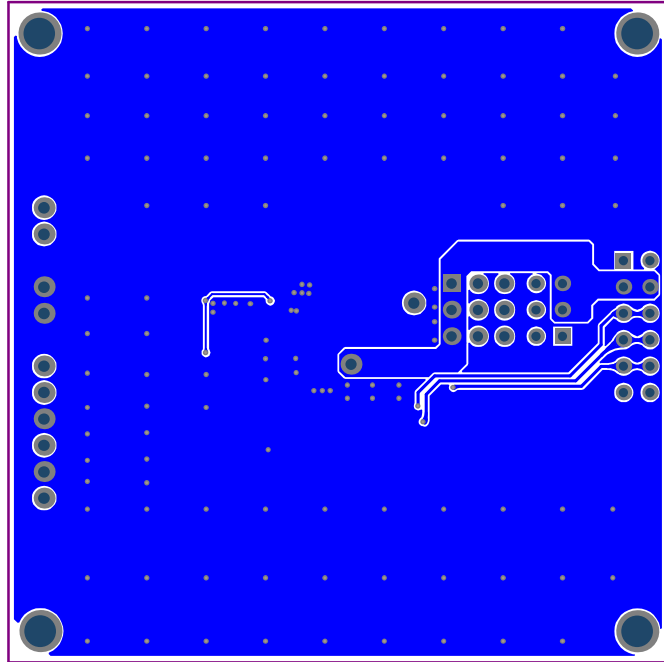
Figure 5: Bottom Layer
