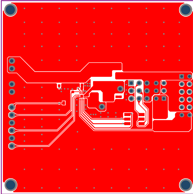
Figure 4: Top Layer
