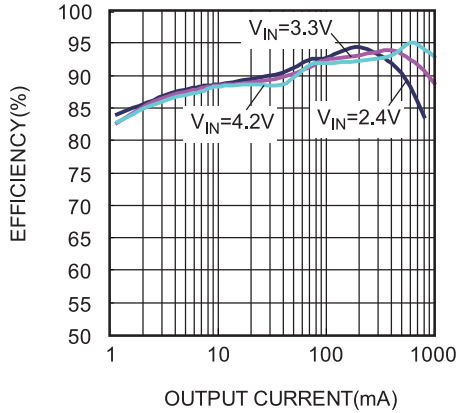
Efficiency vs. Output Current MODE=LOW
