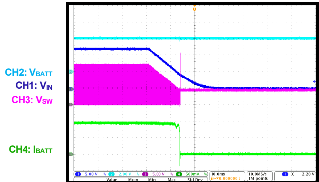
VIN Powers Off Slowly
