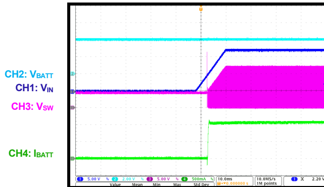
VIN Powers On Slowly
