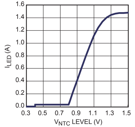
NTC Curve
