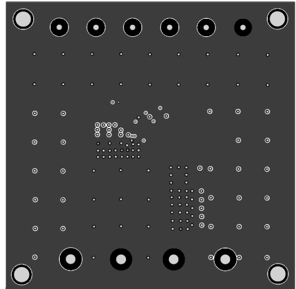
Figure 2: Inner Layer 1
