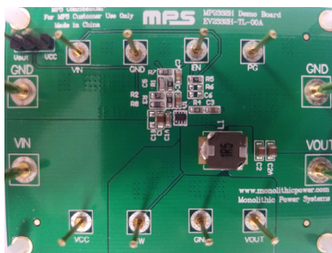
(L x W x H) 63.7mm x 48.4mm x 6.4mm
