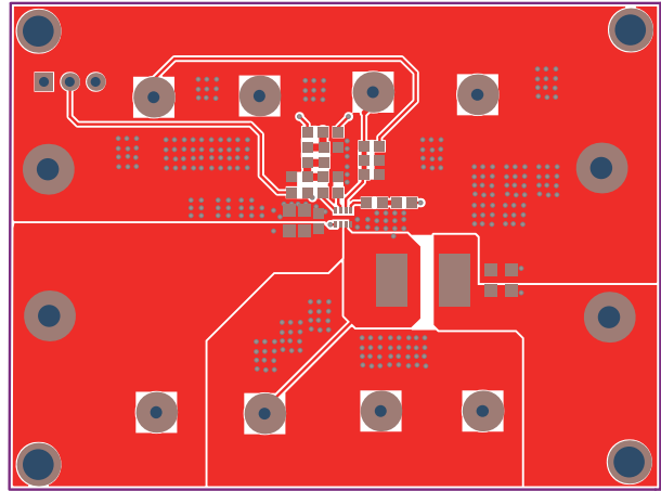
Figure 2: Top layer
