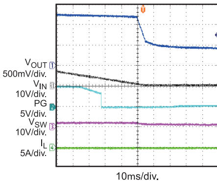
Shutdown through VIN Auto PFM/PWM, I_{OUT}=0A
