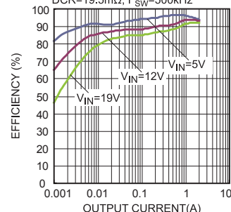
Efficiency vs. Output Current
