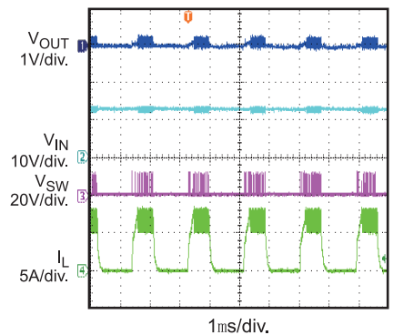
Short-Circuit Steady
