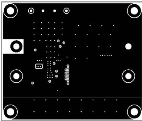
Figure 3—Inner Layer 1
