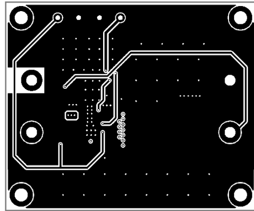
Figure 4—Inner Layer 2
