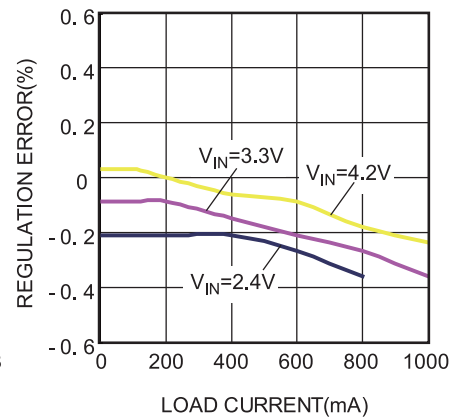
Load Regulation MODE=HIGH
