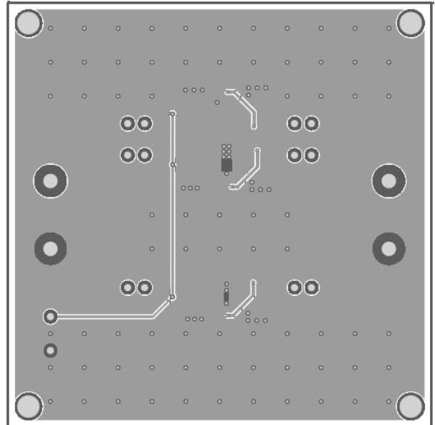
Figure 2 – Bottom Layer
