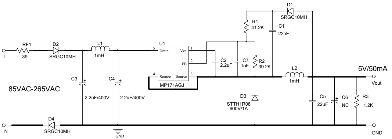
Figure 1: Schematic
