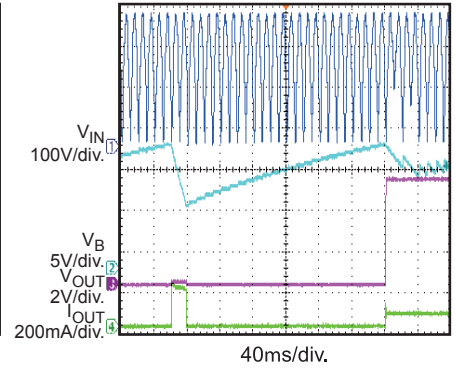
Short Circuit Protection Recovery 230Vac
