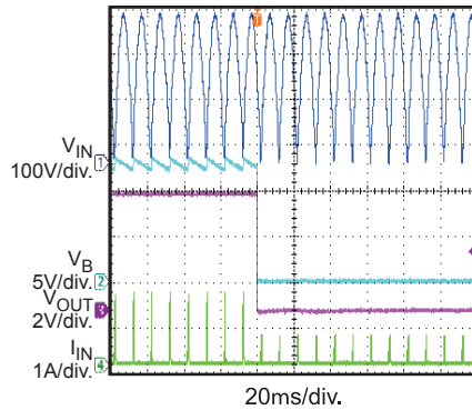
VB Short to GND Protection Entry 230Vac
