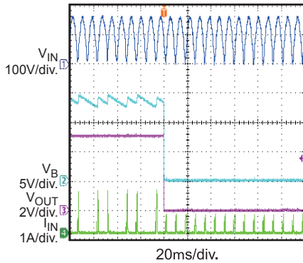
VB Short to GND Protection Entry 115Vac
