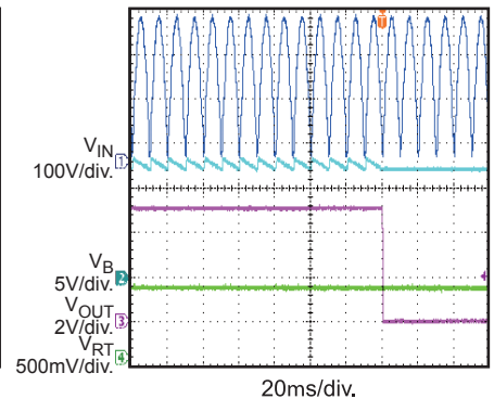
RT Protection Entry 230Vac
