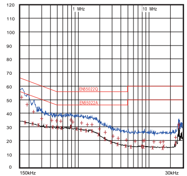
EMI Performance
