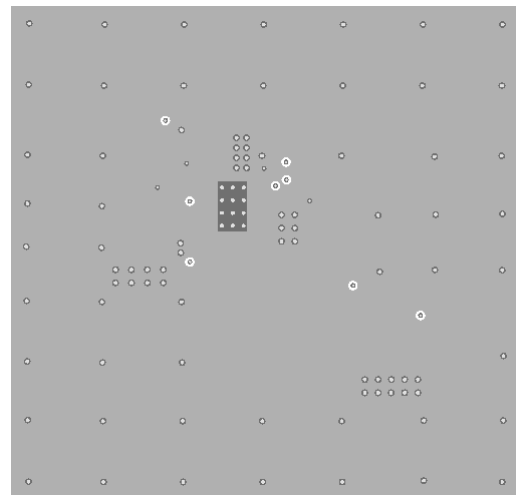
Figure 3 – Recommended PCB Layout
