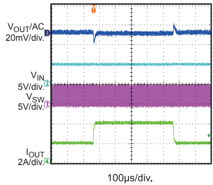
Load Transient Response I_{OUT} = 2A-4A , PFM
