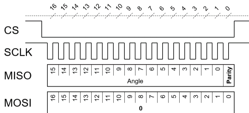
Figure 18: SPI Angle Reading with Parity Bit
