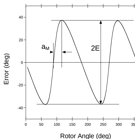
Figure 22: Error Curve in Side-Shaft Configuration with BCT = 0
