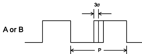
Figure 29: ABZ Jitter
