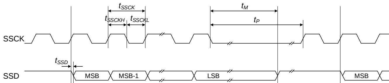
Figure 15: SSI Timing
