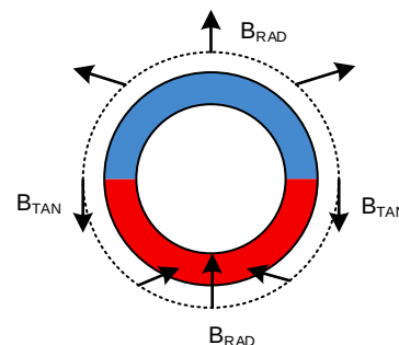
Figure 20: Side-Shaft Field
