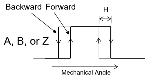
Figure 28: Hysteresis of the Incremental Output
