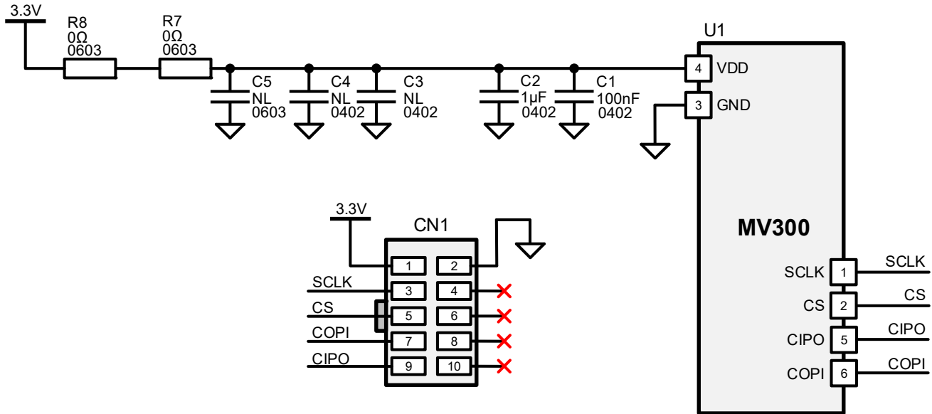
Figure 6: TBMV300-Q-LT-SPI Schematic
