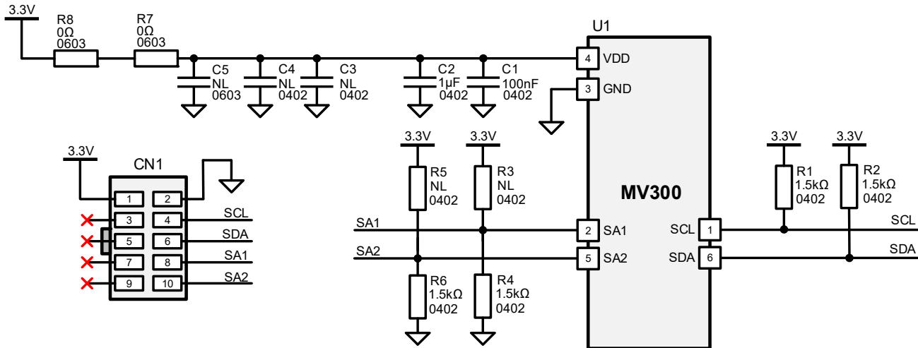
Figure 4: TBMV300-Q-LT-I2C Schematic
