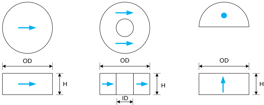
Figure 36: MPS's MAG10 Magnet Geometries
